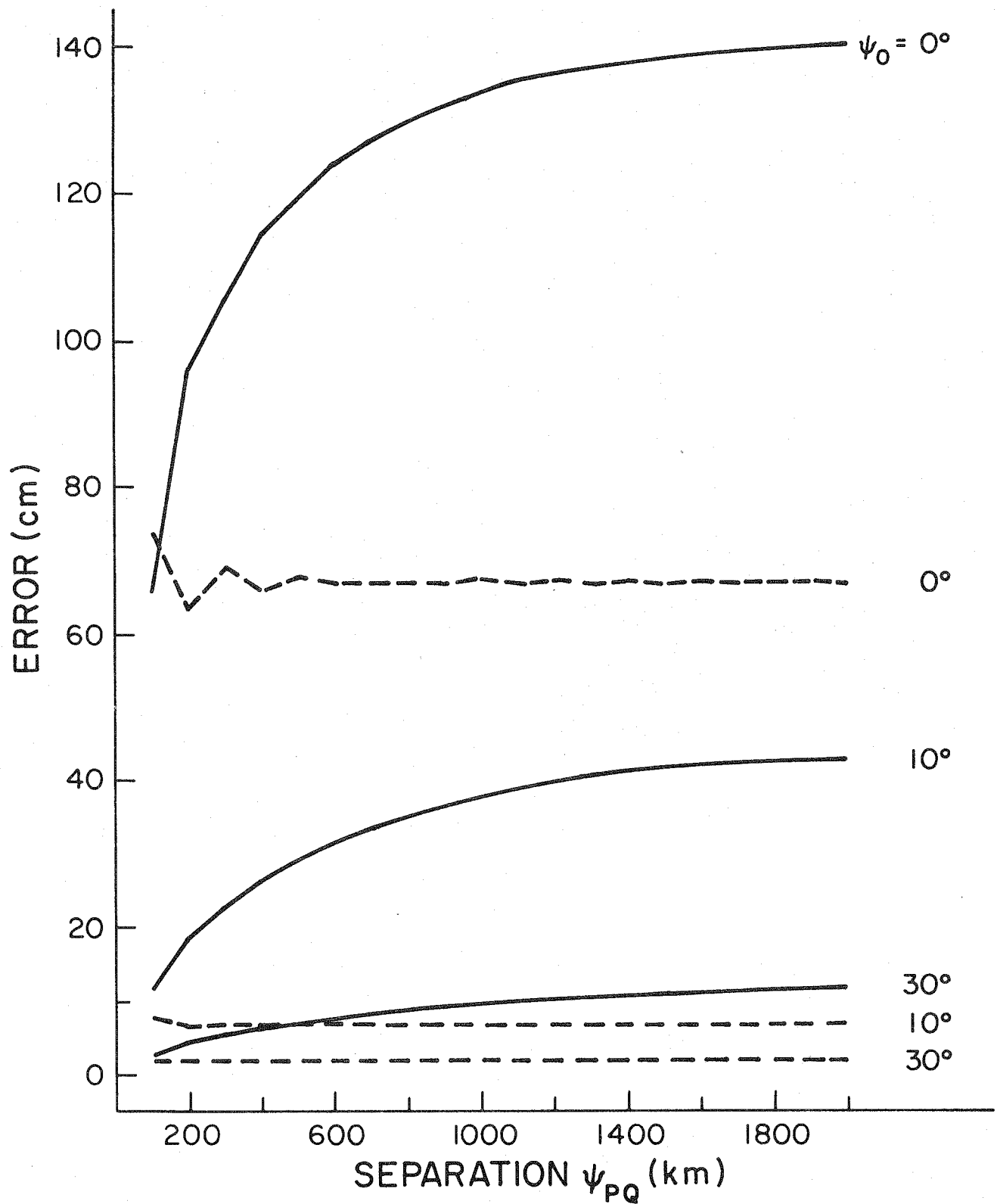
Figure 4. Commission (Solid line) and Truncation (Dotted line) Undulation Difference Errors Assuming Perfect Gravity Anomaly Data Within a Cap of Radius \psi_0 and Potential Coefficients Estimated to Degree 180.
