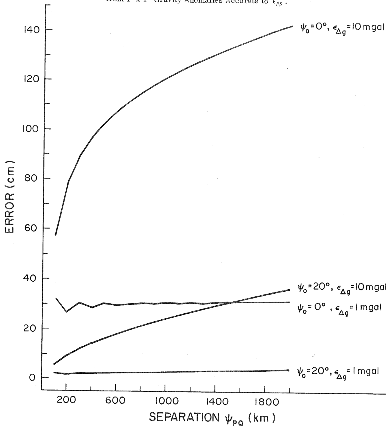
Figure 8. Total RMS Errors for 1^\circ \times 1^\circ Mean Undulation Differences, Assuming Perfect Gravity Anomaly Data Within a Cap of Radius \psi_0 and Potential Coefficients to Degree 180 Estimated from 1^\circ \times 1^\circ Gravity Anomalies Accurate to \epsilon_{\Delta g} .
