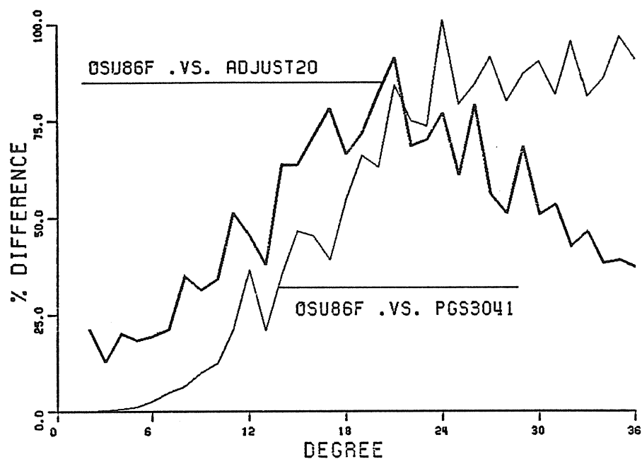
Figure 35. Percentage Differences Between OSU86F Versus ADJUST20 and OSU86F Versus PGS3041.
