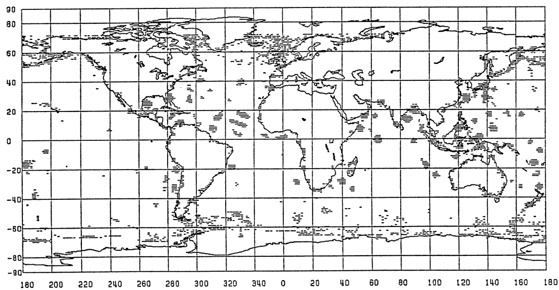
Figure 29. Locations of the 3574 1°x1° Blocks Where |\bar{\Delta g}_{GEM} - (\bar{\Delta g}_{alt} - hf_5)| > 10 mgals.
