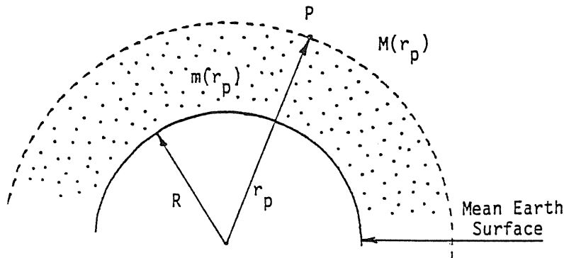
Figure 6. Atmospheric Correction.
