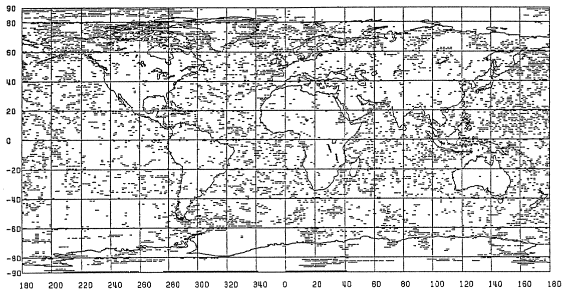
Figure 25. Locations of the 10149 1^\circ \times 1^\circ Blocks Where Condition (5.19) is Fulfilled. (Locations Corresponding to Geophysical Data are Included in the Comparison).
