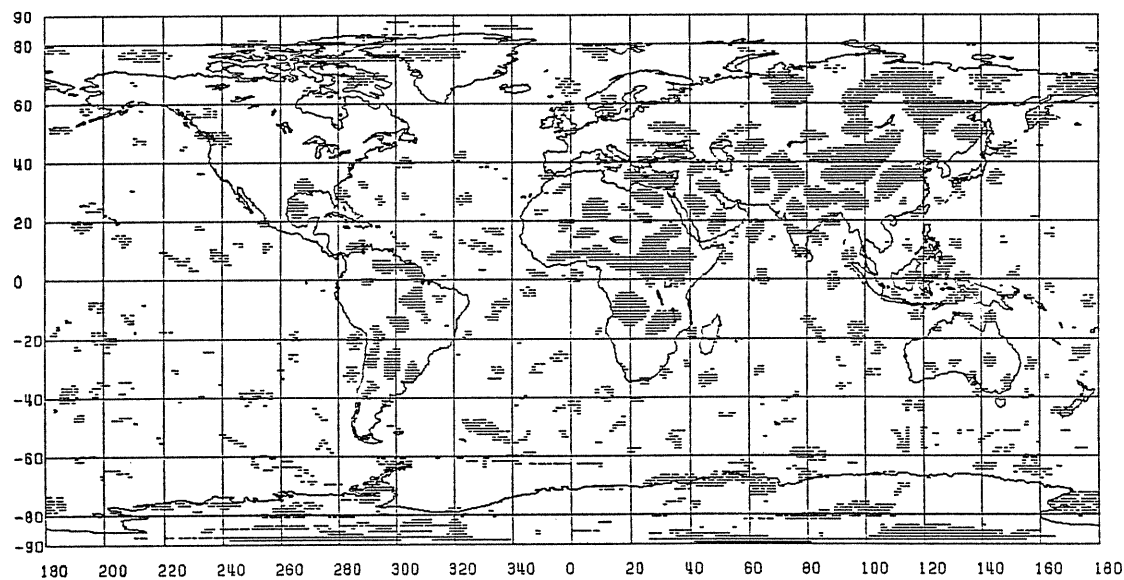
Figure 26. Locations of the 6933 1^\circ \times 1^\circ Blocks Where Condition (5.20) is Fulfilled. (Locations Corresponding to Geophysical Data are Included in the Comparison).
