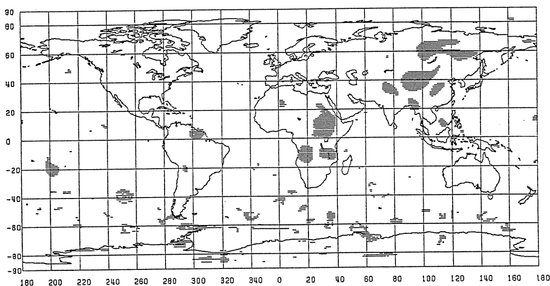
Figure 38. Locations of the 2550 1^{\circ} \times 1^{\circ} Blocks Where |\bar{\Delta}g_{1^{\circ} \times 1^{\circ} OSU86F_{2 \rightarrow 36}} - \bar{\Delta}g_{1^{\circ} \times 1^{\circ} ADJUST_{20}}| > 10 \text{ mgals} .
